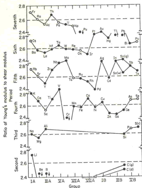
FIG. 23. The ratio of Young's modulus to the shear modulus of all of the elements considered in this review with the exception of the rare-earth elements. The horizontal dashed line represents the mean value of this ratio for these elements. Open points are estimated values.
